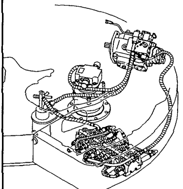
Fig. 74 油圧配管 (走行) HYD. OIL PIPING (TRAVEL)
